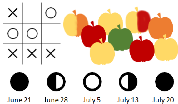
Figure 1: Simple examples of distributions. Top left: a distribution of symbols over a grid in a tic-tac-toe game. Top right: a distribution of colours over a set of apples. Bottom: a distribution of the shapes of the moon over time.
